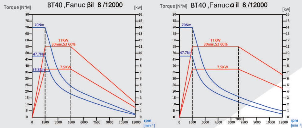
HMC- 400 BT40 Direct Type 12000rpm
