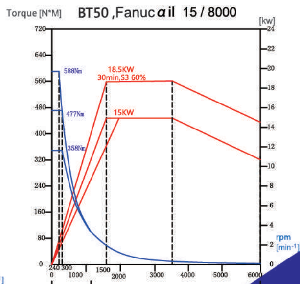
HMC- 500/630 BT50 1 : 5 GEAR HEAD
