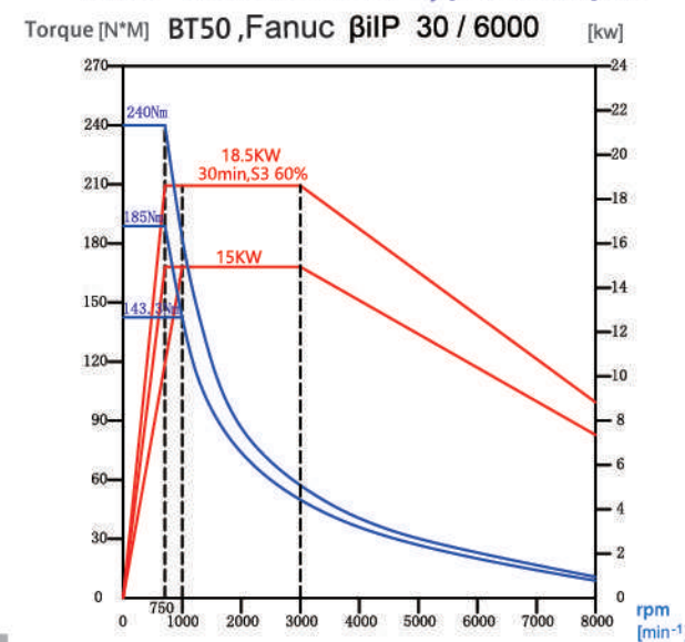
HMC- 630 BT50 Belt Type 6000rpm
