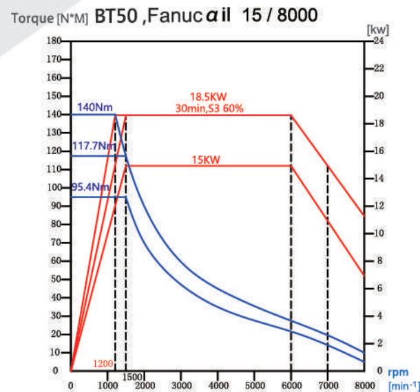
HMC- 500/630 BT50 Belt Type 8000rpm
