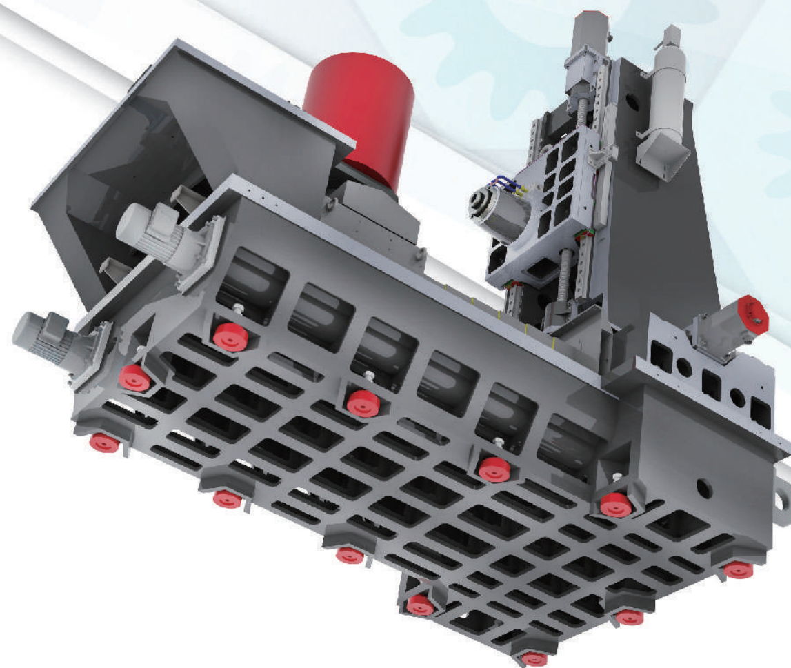
HMC-500-BASE SimulationXpress Study Stress Analysis 1.48993e+010
